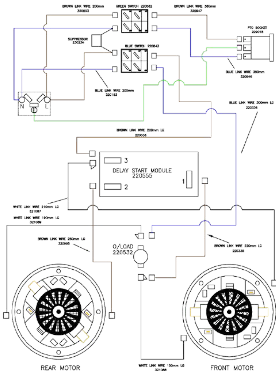
Wiring Diagram
