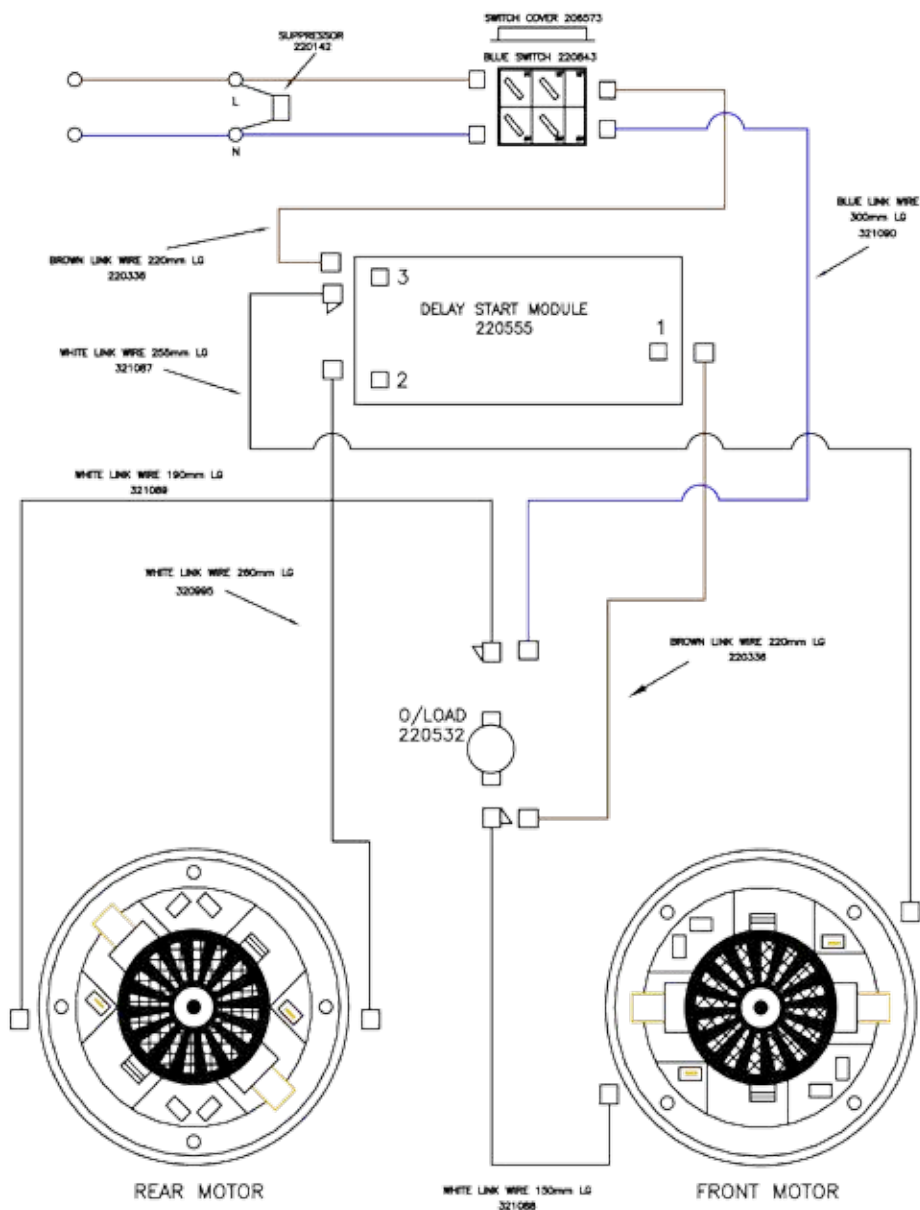
Wiring Diagram
