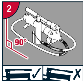
Place Hydraulic Assembly on ground in horizontal position.
