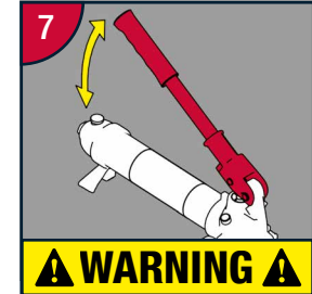
Pump the handle just enough to free up the collar. Do not over-pump.
