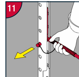
Whilst holding the hose , remove the ram securing pin.
