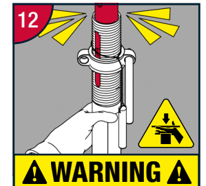
Continue to support outer tube and lower the hose. Be aware of trap/crush injuries.
