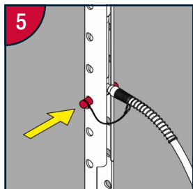
Insert ram securing pin through first available hole directly beneath the ram.
