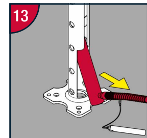
Continue to support outer tube and remove ram via ram access chamber.
