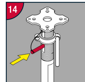
Replace top pin through available hole below collar and the removal is complete.
